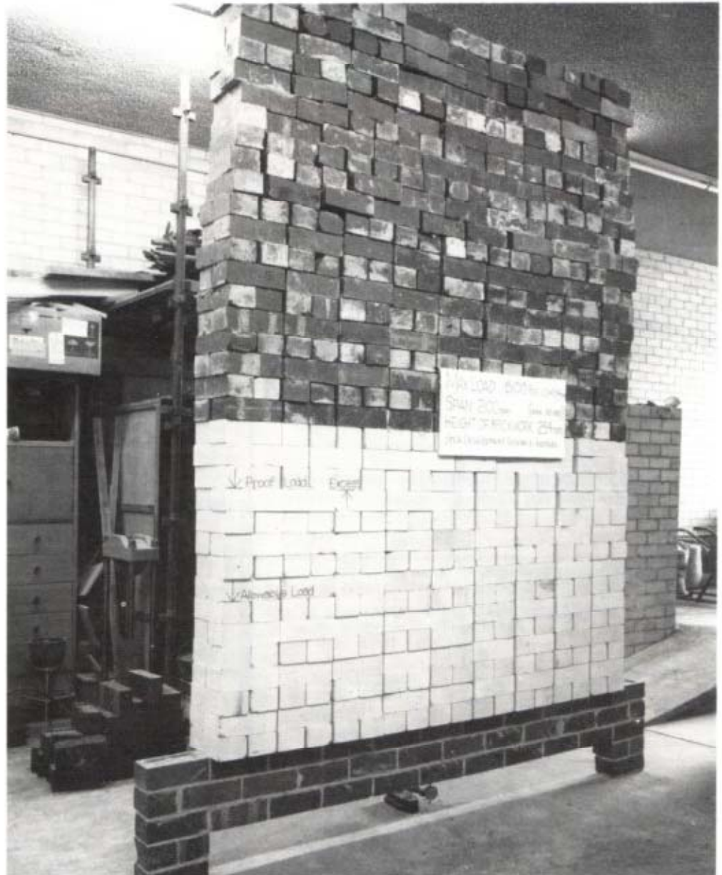
A HESBIA lintel of 2100mm clear span under test at the Brick Development Research Institute. Bricks were used to load the beam to show that long-term creep deflection is small.
